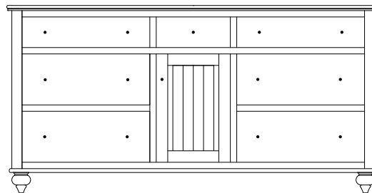
WB-1756 Dresser 73"w 36¾"h 21"d w/7 drawers, 1 door w/1 adjustable shelf
