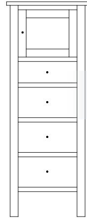
CA-547 Lingerie 23"w 60¼"h 21½"d w/4 drawers, 1 wood door, 1 adjustable shelf
