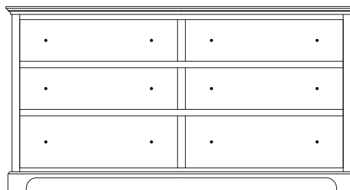
SO-131 Dresser 67¾"w 35½"h 21"d w/6 drawers
