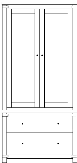
LN-2362 Armoire 35 \frac{1}{4} "w 75"h 19 \frac{3}{4} "d w/2 drawers, (top drawer w/divider) w/2 doors, 2 adj. shelves & closet rod
