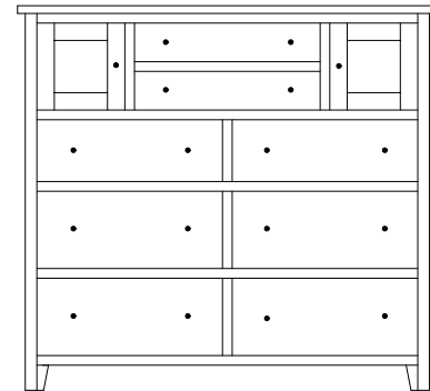
OD-2753 His & Hers Chest 54¼"w 49¾"h 21½"d w/8 drawers, 2 doors
