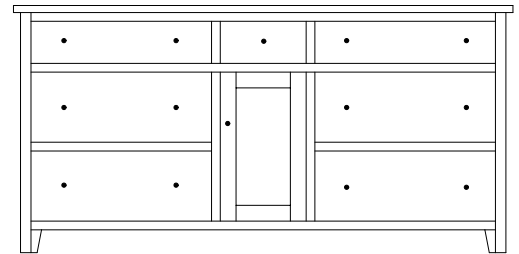
OD-2756 Dresser 71 \frac{1}{4} "w 35 \frac{1}{4} "h 21 \frac{1}{2} "d w/7 drawers, 1 door w/1 adjustable shelf
