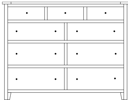
TM-3357 Dresser 57 \frac{3}{4} "w 44 \frac{3}{4} "h 21 \frac{1}{2} "d w/9 drawers
