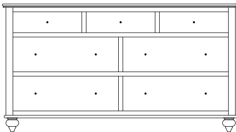
WB-1755 Dresser 67¾"w 36¾"h 21"d w/7 drawers
